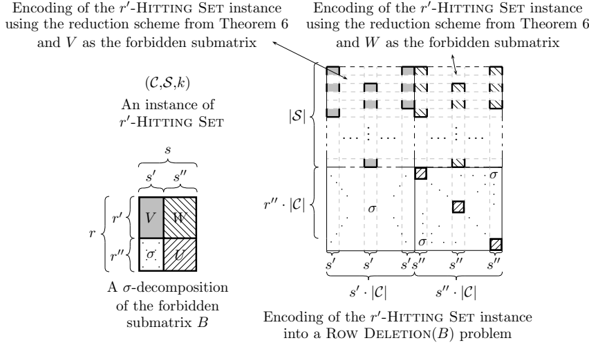
Figure 5: Reduction from r' -HITTING SET to ROW DELETION( B ) used in the proof of Theorem 4.
