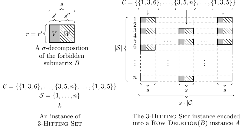
Figure 3: An example reduction from 3-HITTING SET to ROW DELETION( B ) following from the proof of Theorem 6 (illustrated for the case where r' = r ).
