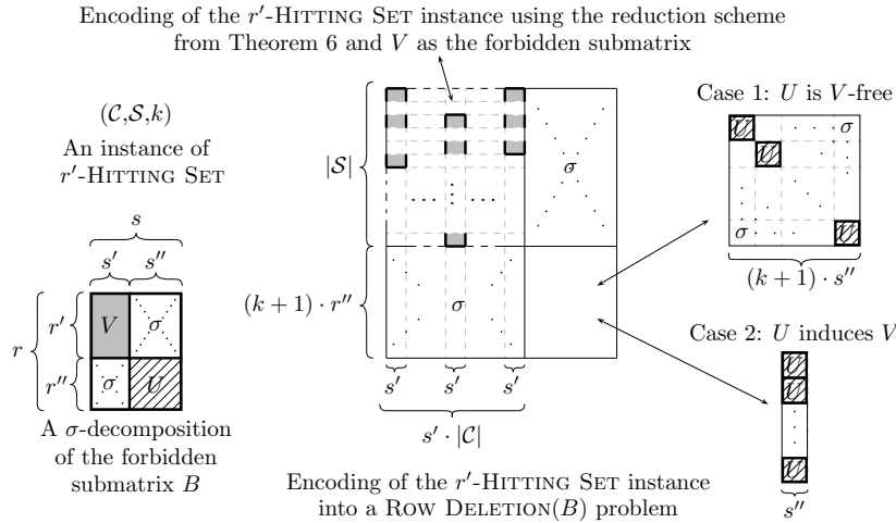
Figure 4: Reduction from r' -HITTING SET to ROW DELETION( B ) used in the proof of Theorem 7.
