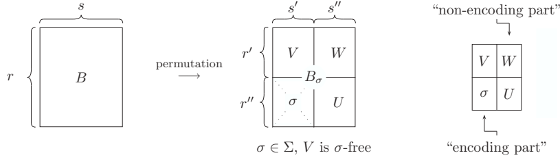
Figure 2: General scheme for the \sigma -decomposition of a matrix B over the alphabet \Sigma .
