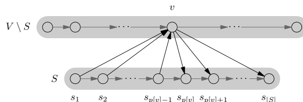
Fig. 2. Illustration of equivalence (1). For clarity, only some of the arcs are shown.
