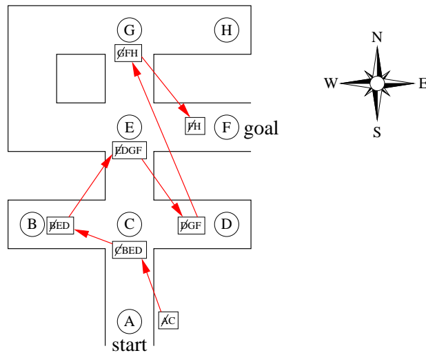
Fig. 1.8 Example for breadth-first search in the labyrinth
